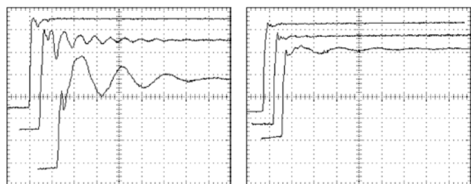
a. Passive probe.
